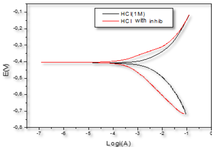
Fig 1 : Polarization curves of X70 steel in HCl medium (1M) without and with the inhibitor.
